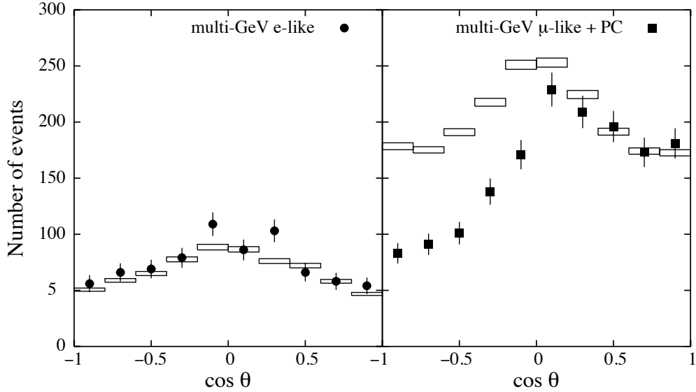
Figure 24.7: Zenith-angle dependence of multi-GeV neutrino interactions from SuperKamiokande [68]. The shaded boxes show the expectation in the absence of any oscillations.
