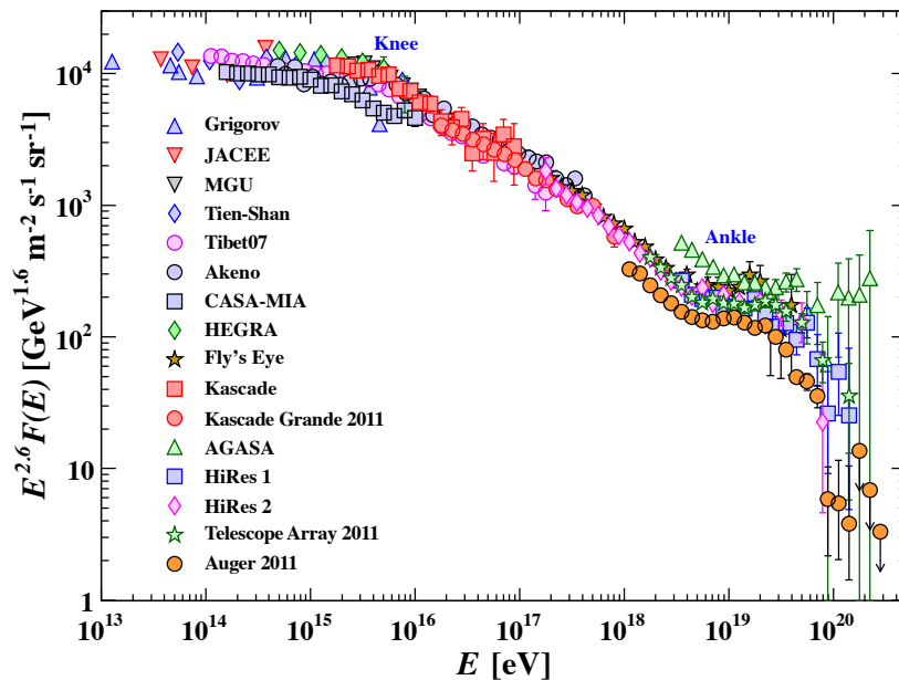
Figure 24.8: The all-particle spectrum as a function of E (energy-per-nucleus) from air shower measurements [79–90,100–104]. Color version at end of book.
