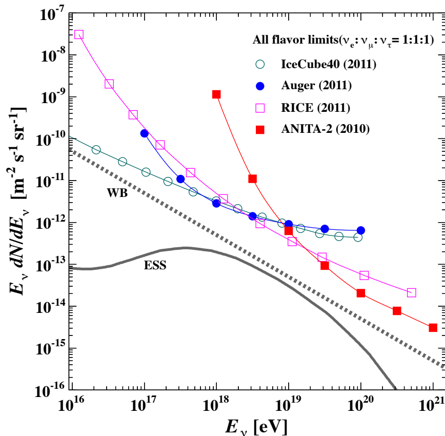
Figure 24.10: Differential limits on the flux of cosmogenic neutrinos set by four neutrino experiments. The curves show the Waxman-Bahcall benchmark flux (WB, [111]) and a representative midrange model for the expected flux of cosmogenic neutrinos (ESS, [110]). The expected flux is uncertain by over an order of magnitude in either direction.
