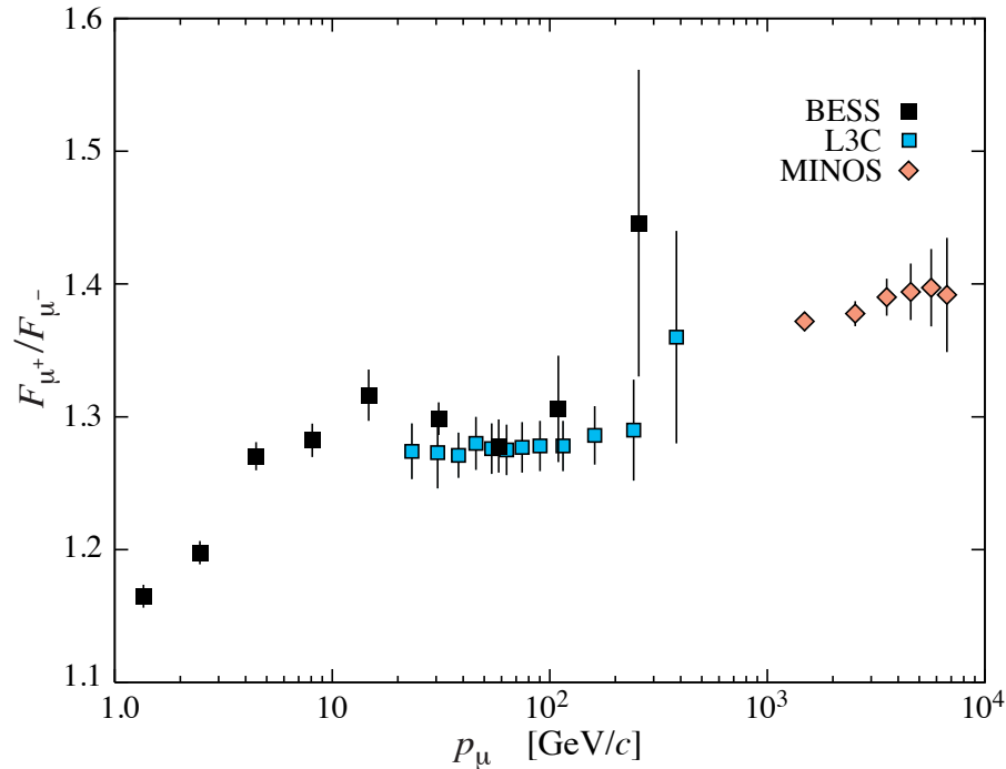
Figure 24.5: Muon charge ratio as a function of the muon momentum from Refs. [44,45,51].
