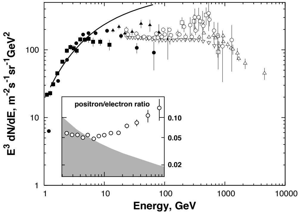
Figure 24.2: Differential spectrum of electrons plus positrons multiplied by E^3 (data from [17–23]). The line shows the proton spectrum multiplied by 0.01. The inset shows the positron to electron ratio measured by PAMELA [24] compared to the expected decrease [25].
