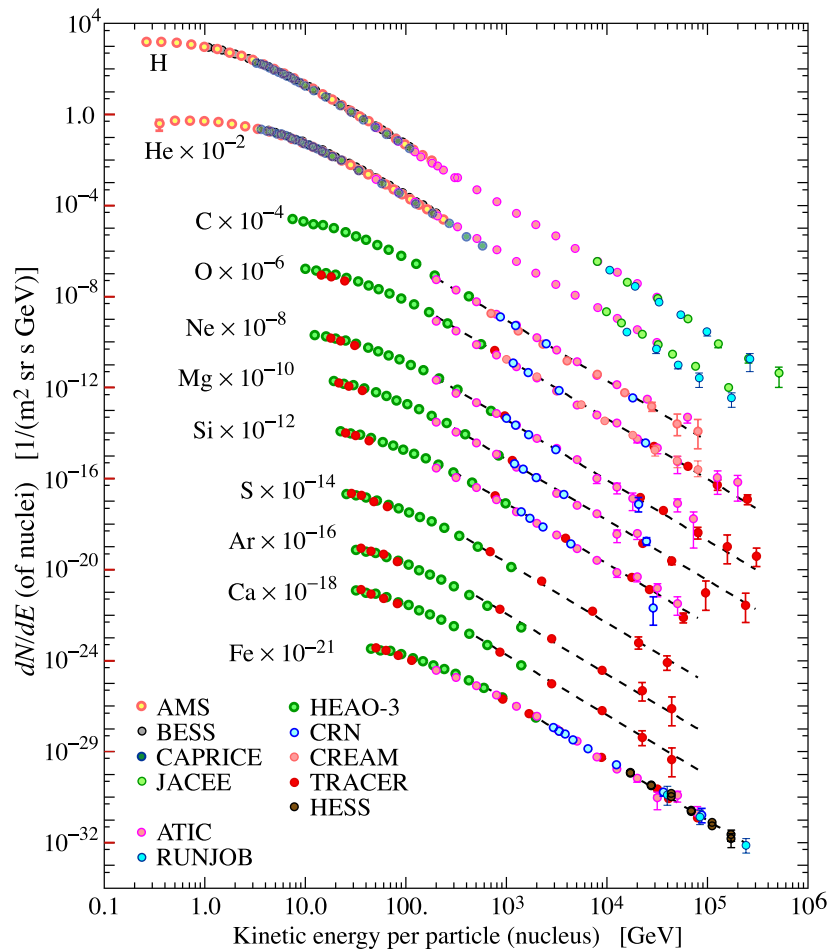
Figure 24.1: Fluxes of nuclei of the primary cosmic radiation in particles per energy-per-nucleus are plotted vs energy-per-nucleus using data from Refs. [1–12]. The figure was created by P. Boyle and D. Muller. Color version at end of book.
