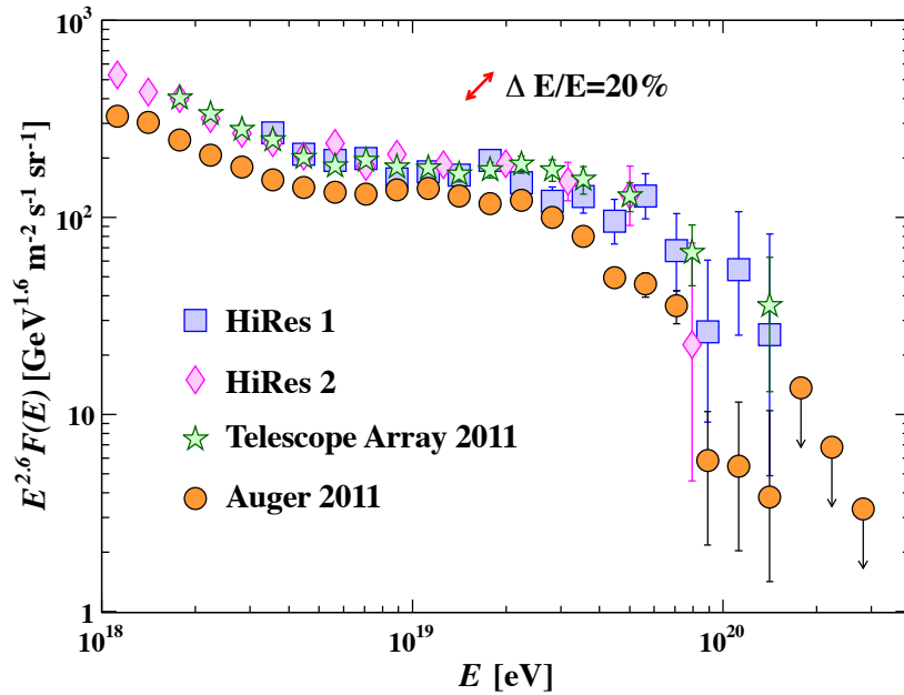
Figure 24.9: Expanded view of the highest energy portion of the cosmic-ray spectrum from data of HiRes 1&2 [101], the Telescope Array [103], and the Auger Observatory [104]. The HiRes stereo spectrum [112] is consistent with the HiRes 1&2 monocular results. The differential cosmic ray flux is multiplied by E^{2.6} . The red arrow indicates the change in the plotted data for a systematic shift in the energy scale of 20%.
