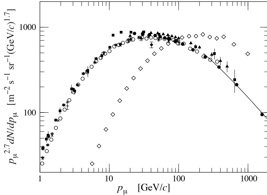
Figure 24.4: Spectrum of muons at \theta = 0^\circ ( \diamond [41], \blacksquare [46], \blacktriangledown [47], \blacktriangle [48], \times , + [43], \circ [44], and \bullet [45] and \theta = 75^\circ \diamond [49]). The line plots the result from Eq. (24.4) for vertical showers.
