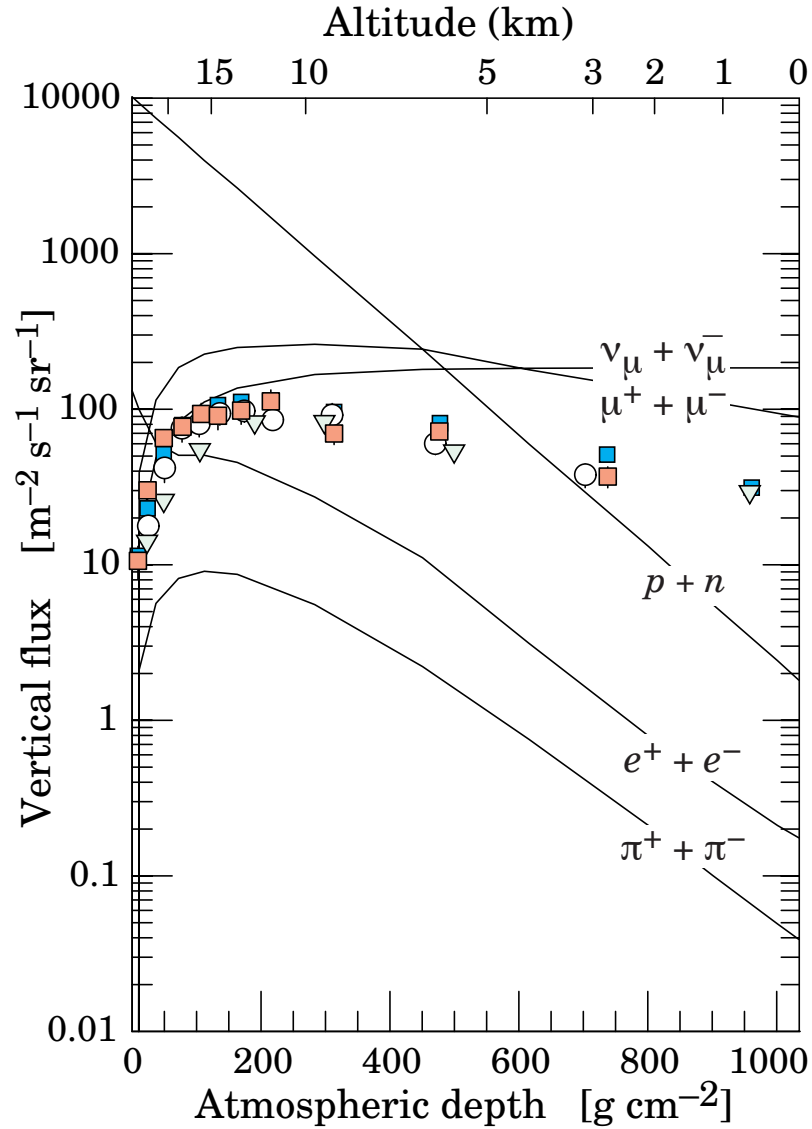
Figure 24.3: Vertical fluxes of cosmic rays in the atmosphere with E > 1 GeV estimated from the nucleon flux of Eq. (24.2). The points show measurements of negative muons with E_\mu > 1 GeV [32–36].
