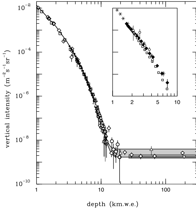
Figure 24.6: Vertical muon intensity vs depth (1 km.w.e. = 10^5 g cm ^{-2} of standard rock). The experimental data are from: \diamond : the compilations of Crouch [58], \square : Baksan [63], \circ : LVD [64], \bullet : MACRO [65], \blacksquare : Frejus [66], and \triangle : SNO [67]. The shaded area at large depths represents neutrino-induced muons of energy above 2 GeV. The upper line is for horizontal neutrino-induced muons, the lower one for vertically upward muons. Darker shading shows the muon flux measured by the SuperKamiokande experiment. The inset shows the vertical intensity curve for water and ice published in Refs. [59–62].
